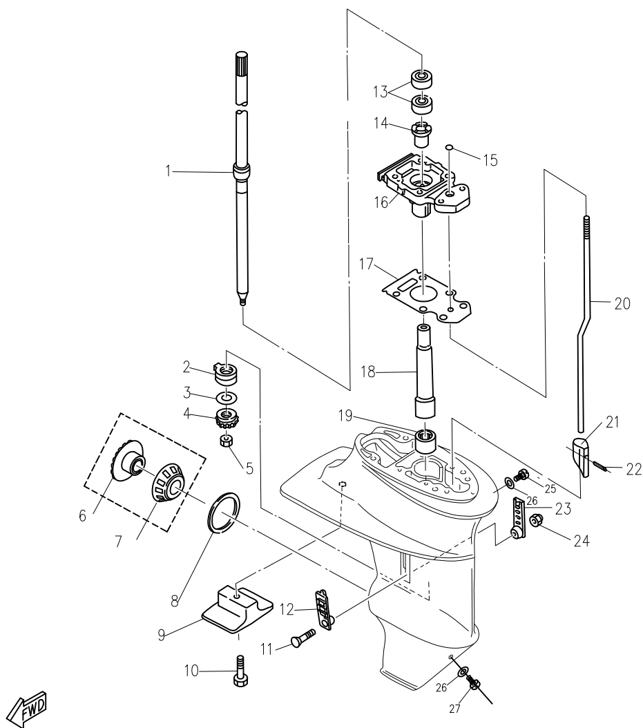
FIG. 16 DRIVE SHAFT, FORWARD GEAR AND SHIFT ROD 图16 驱动轴，正挡齿轮和变挡连杆
