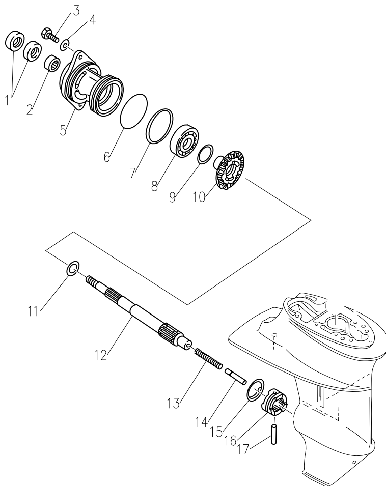
FIG. 17 PROPELLER SHAFT AND REVERSE GEAR 图17 螺旋桨轴和倒挡齿轮
