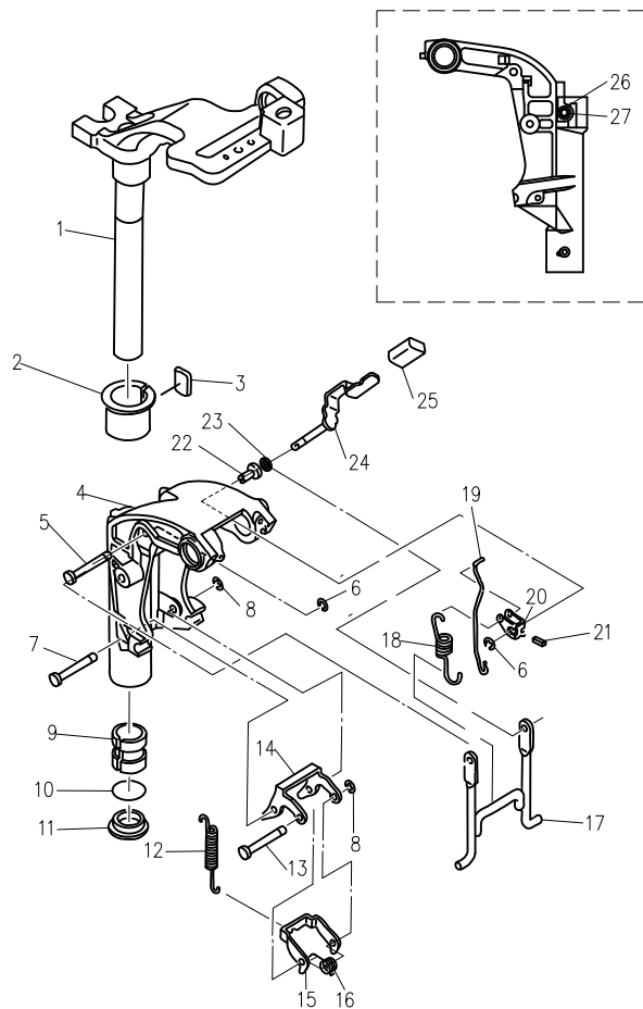
FIG. 12 STEERING AND SWIVEL BRACKET 图12 操舵与旋转支架
